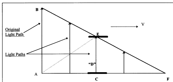
Fig 4 Current physics says that AE is the path that light follows to the upper mirror and the angle of this path is depended on the length AC that is depended on the speed of the light clock.
