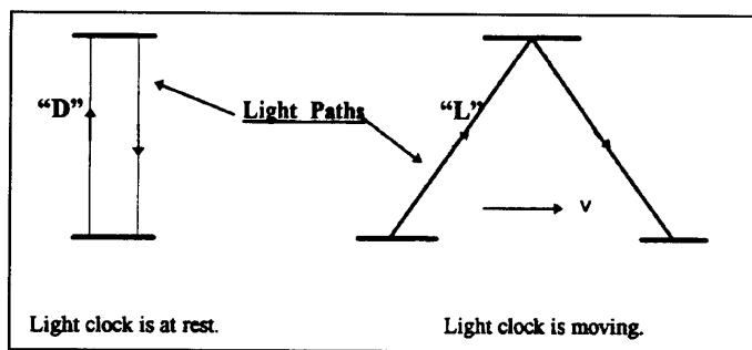
Fig 3 Light paths in a light clock at rest and in motion.
