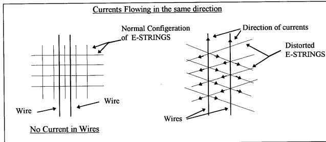
Figure 1. Currents (electrons) in the wires are flowing in the same direction, and therefore the force between the electrons is attractive. The right diagram that shows that the tension created in the E-Strings by the absolute motions of the electrons is pulling the wires together.
