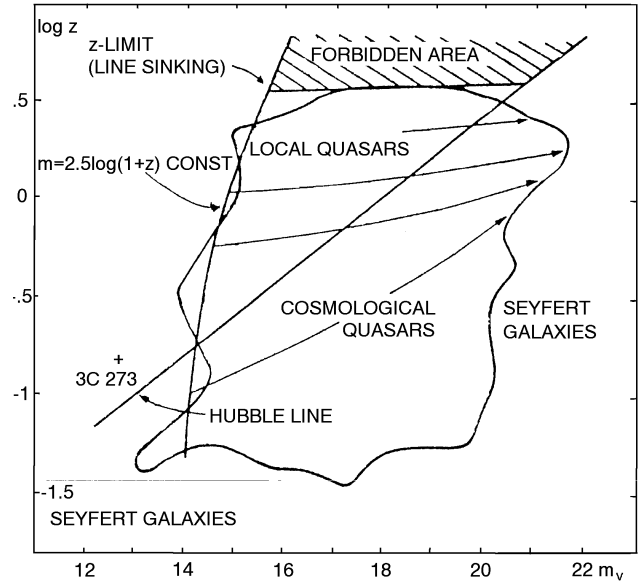
Figure 2. Interpretation of the Hubble diagram of quasars. The QSOs are within the wavy outline. The Hubble line is drawn through the QSOs with z equal to that of a nearby galaxy. The quasars on the left side edge of the distribution are the nearest ones, with z almost totally non-cosmological. The curved arrows show the distance effect for such QSO redshifts; note the accumulation in the upper right corner where there is also an extension in the observed distribution. Position of the QSOs vs. Type 1 Seyfert galaxies is due to distance-dependent morphology. Other details are apparent from the figure and from the text.
