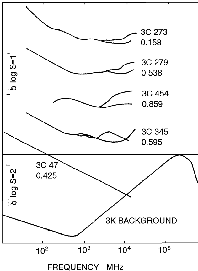
Figure 1. Illustrates a spectral relationship between quasars and the background radiation. Four upper curves are for flat spectrum (i.e. non-cosmological QSOs), with the branches showing the variable spectra 1-3 years apart. Note the beginning of the flattening at the same frequency as where the 3 rd spectrum begins to rise. The straight, steep spectrum is probably for a cosmological QSO. The redshifts of the QSOs are given.
