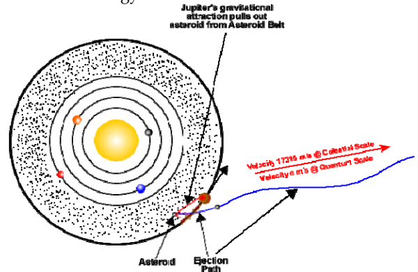
Fig. 17.2. Celestial Photon Ejection
