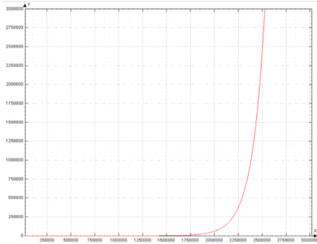
Fig. 14.2. \lambda where object accelerates away from all matter into absolute-ly empty space
