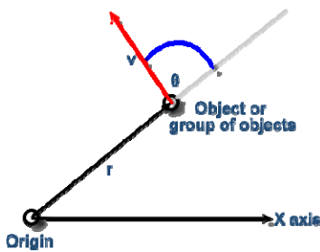
Fig. 9.1. Measurement of change via angular velocity
