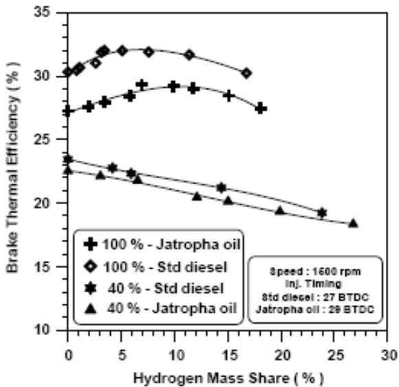
Fig. 4. Variation of thermal efficiency with hydrogen mass share [6]
