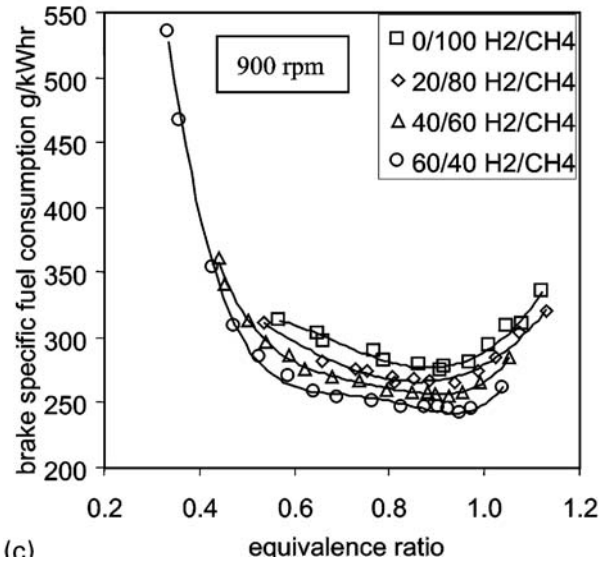
Fig. 5. Reduction in fuel consumption with increase in hydrogen addition [3]
