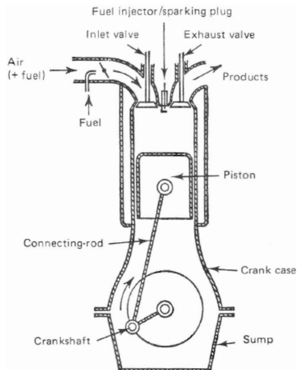
Fig. 1. Four Stroke Internal Combustion Engine [1]
