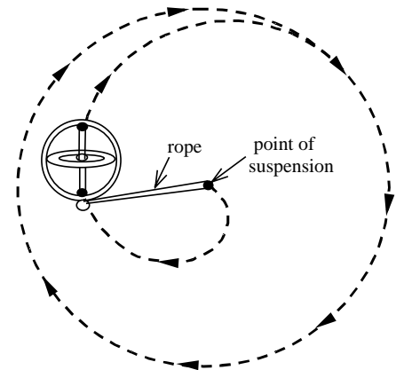
Fig. 4.20 A gyro tethered to the roof (over 50 feet high) orbiting (plan view)
