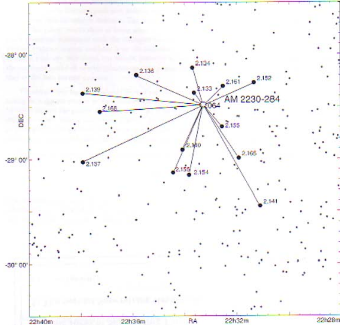
Fig. 3.— An Unprecedentedly Large Quasar Family. All quasars in a 3 \times 3 degree 21F field are plotted as filled circles. Inside 70'' and for z between 2.125 and 2.175, the filled circles are larger and labeled with redshifts. Diagram courtesy D. Carosati.
