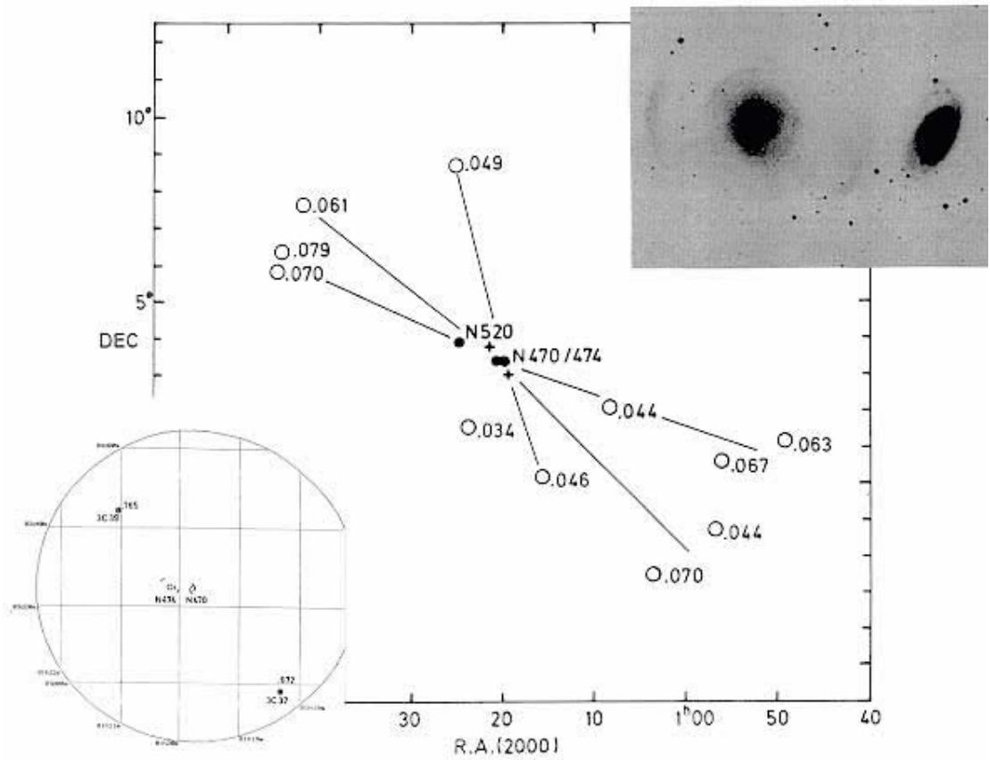
NGC 470/474 (ARP 227), TWO DISTURBED GALAXIES WITH A PAIR OF STRONG RADIO QUASARS (3C 37 AND 3C 39) PAIRED ACROSS THEM. ACCIDENTAL PROBABILITY OF THIS ALIGNMENT IS 2 \times 10^{-9} . BRIGHT ABELL CLUSTERS BETWEEN 15.0 \leq m_{10} \leq 16.4 mag. FALL ALONG EJECTION LINE DEFINED BY QUASARS.
