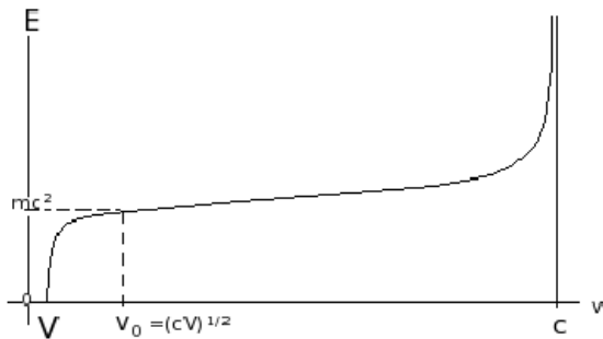
FIG. 3: v_0 represents the speed in relation to S_V , from where we get the proper energy of the particle ( E_0 = mc^2 ), being \Psi_0 = \Psi(v_0) = 1 . For v \ll v_0 or closer to S_V ( v \rightarrow V ), a new relativistic correction on energy arises, so that E \rightarrow 0 .
