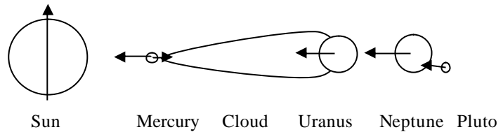
fig.5.1.a : gravitational planet's sepatation model : separation of ME, UR, NE, PL.
