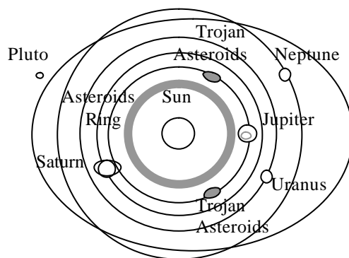
fig.5.5 : orbits of our planetary system.
