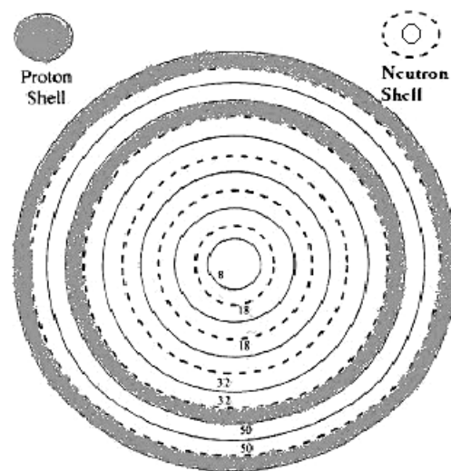
Fig. 1. Cross-sectional view of the electrodynamic shell model of 208 Pb.
