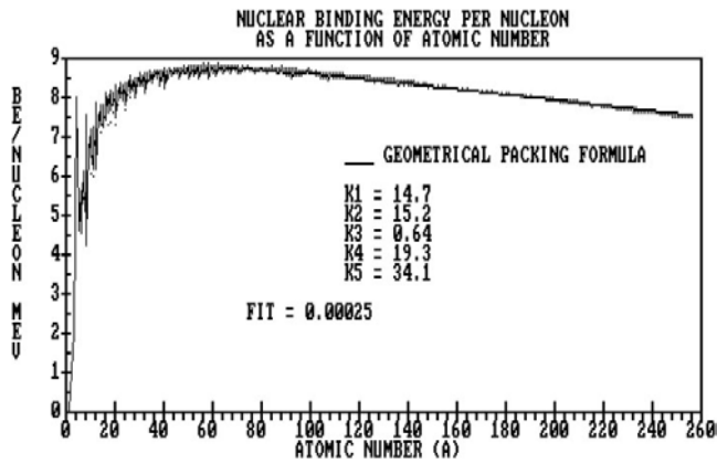
Fig. 2. New semiempirical binding energy fit from the electrodynamic model.
