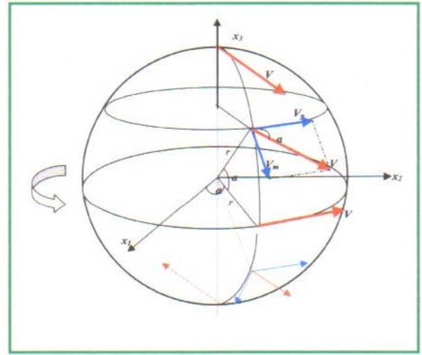
Fig. 4. Geometry of flux velocities in a sample spherical vortex
