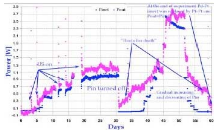
Fig. 2. Excess energy using electrolysis of \text{D}_2\text{O} + \text{LiOD} . Excess energy continued after the power was stopped (heat after death). The amount is in excess of any plausible chemical reaction [34].
