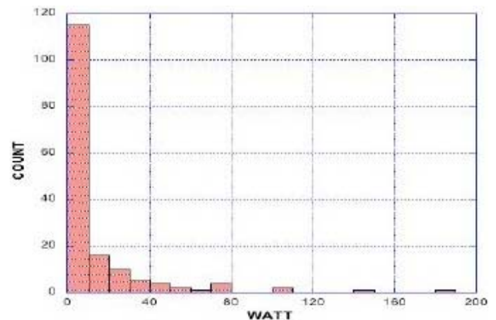
Fig. 1. Histogram of heat production in addition to that applied based on 154 independent measurements [20].
