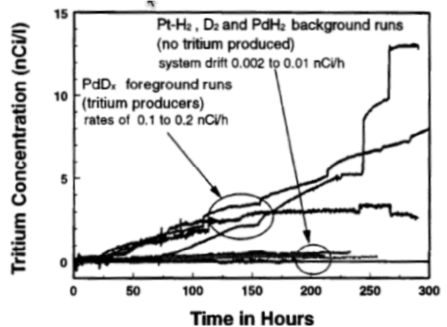
Fig. 6. Production of tritium without neutrons using gas discharge of D 2 . Tritium was measured two different ways [43].
