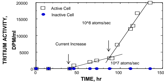
Fig. 3. Tritium production during electrolysis of D 2 O + LiOD [36].
