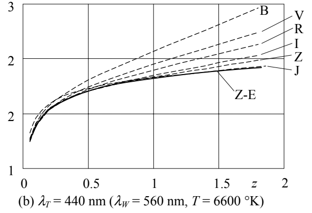
FIG. 3.6-3 (a,b). Magnitudes observed in filters BVRIZJ at distance D = R_4 z / (1+z) from blackbody sources at temperatures 8300 \text{ }^\circ\text{K} and 6600 \text{ }^\circ\text{K} , respectively. (c). Plot of the peak magnitudes of normal Sn Ia observed in BVRIYJ filters as presented by Tonry et al. [13] in Table 7. The transmission functions of the filters used by Tonry et al. are slightly different from the transmission functions used in calculations for (a) and (b). See Appendix B for the definitions of \lambda_T and \lambda_W . The zero-energy prediction (3.5:10) for the magnitudes in optimally chosen filters is shown by the (Z-E) curve in each figure.
